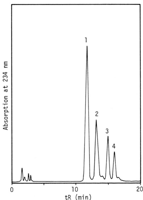
Fig. 1. HPLC of HOM from HPOM produced during incubation of soybean lipoygenase-I with LM at pH 11.0. 1: 13-( Z, E )-HOM; 2: 13-( E, E )-HOM; 3: 9-( E, Z )-HOM; 4: 9-( E, E )-HOM. Analytical conditions: eluting solvent; n -hexane:ethanol = 99.5:0.5 (V/V), 2 ml/min on Zorbax SIL column (4.6 mm \varnothing \times 250 mm) which is packed with silica gel, Shimadzu Dupont Liquid Chromatograph LC-2.
